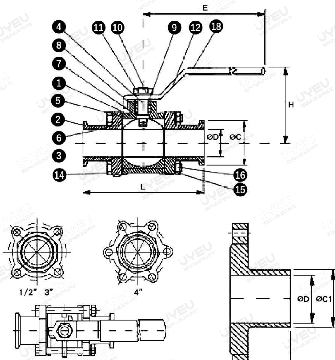
Size Of Clamp & Butt Weld End
